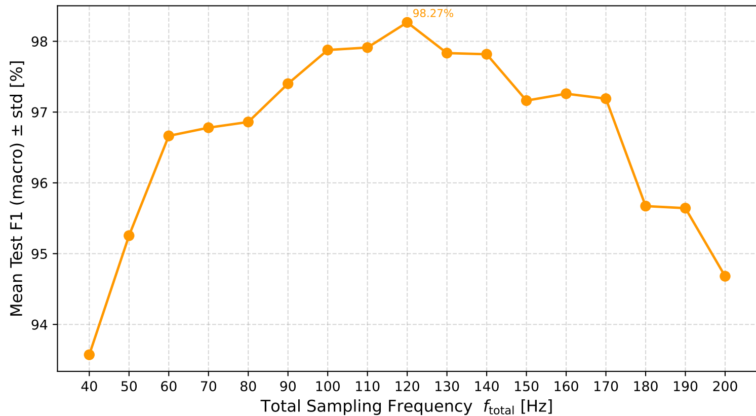
Pareto Curve: Mean F1 across seeds vs. Total Sampling Frequency (Clean→Tremor)
